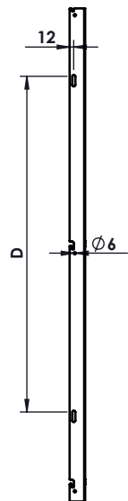
Bracket Assembly
