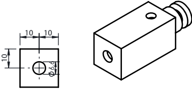
Bracket Assembly
