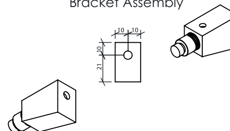
Bracket Assembly
