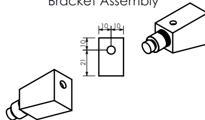
Bracket Assembly
