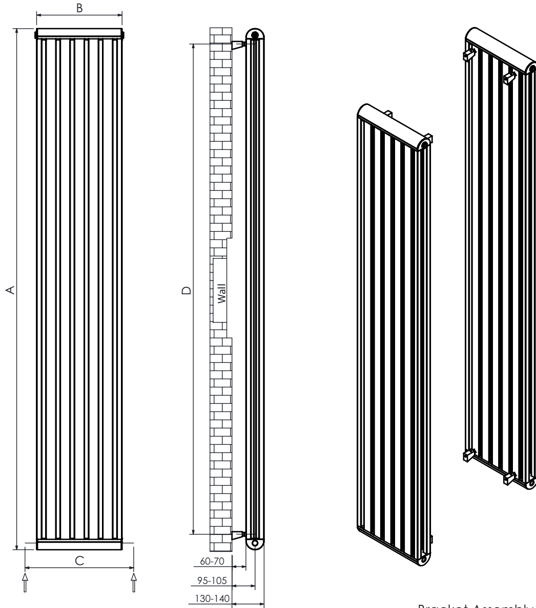
Bracket Assembly
