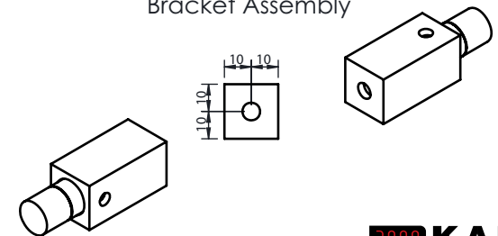
Bracket Assembly
