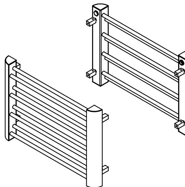
Bracket Assembly
