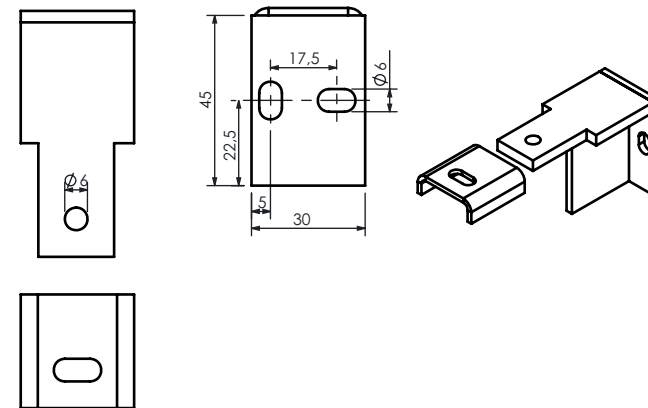
Bracket Assembly
