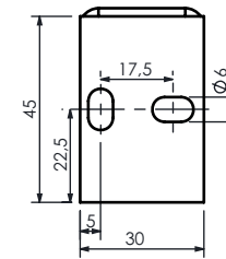
Bracket Assembly
