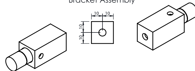
Bracket Assembly
