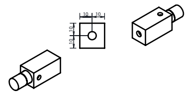
Bracket Assembly
