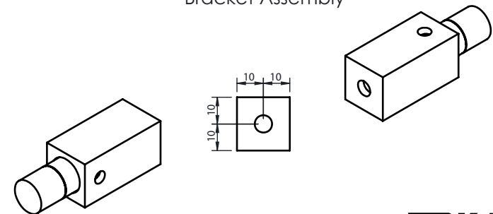
Bracket Assembly
